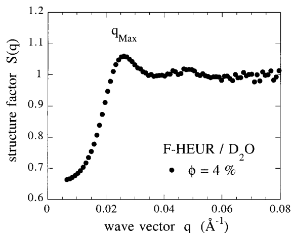
Figure 2. Experimental structure factor S(q) for a F-HEUR solution at \phi = 4\% .
