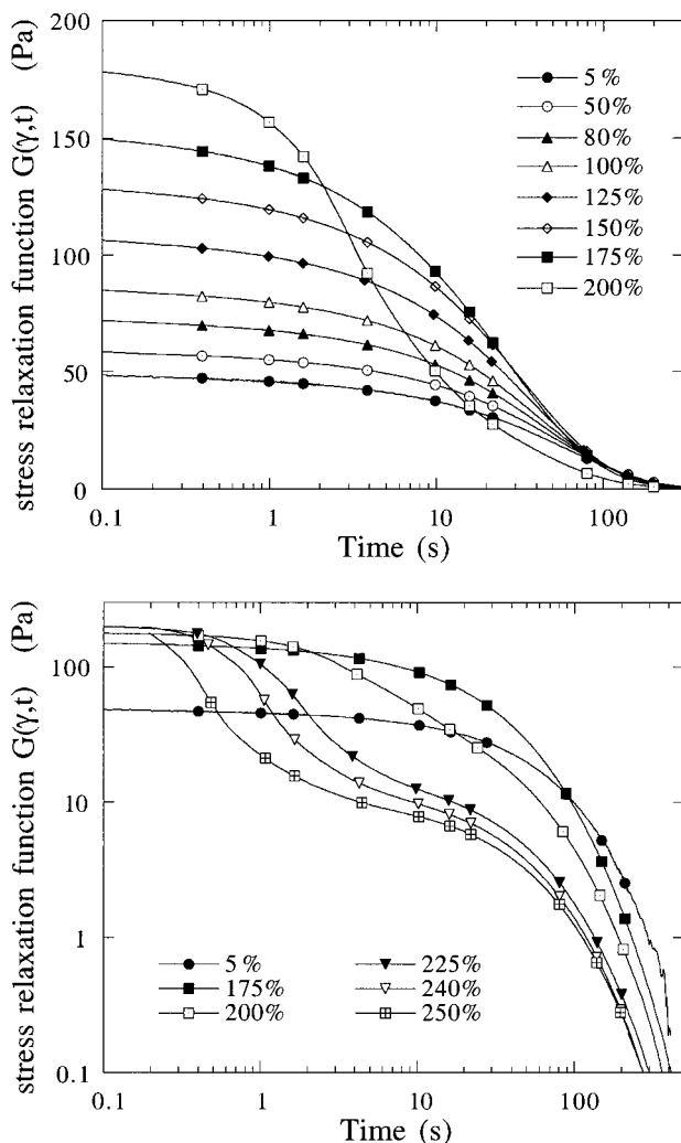
Figure 6. Stress relaxation functions G(t, \gamma) for the F-HEUR/ D_2O solution at \phi = 4\% for strain amplitudes \gamma ranging from 0.05 to 2 (a, top) and from 1.75 to 2.5 (b, bottom) at ambient temperature ( T = 20^\circ C ). Note in (b) the use of a double-logarithmic scale. The response deviates from the linear function G(t, \gamma < \gamma_{lin}) at \gamma_{lin} = 0.4 \pm 0.1 .
